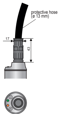
Design „H“ with cable gland for protected hoses – for use in an outdoor environment or in an area with increased moisture.
