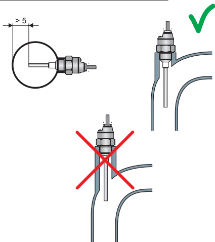
Figure 10: Sensor mounting in a tube
