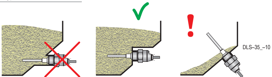
Figure 5: Slant wall mounting
