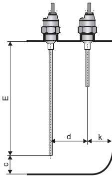
Figure 1: Vertical mounting
