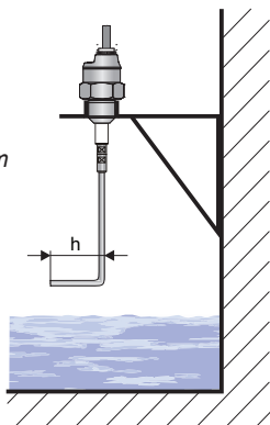
Figure 7: Bending of the electrode end to sense unknown fluids
