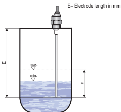
Figure 11: Two-state level regulation by hysteresis setting
